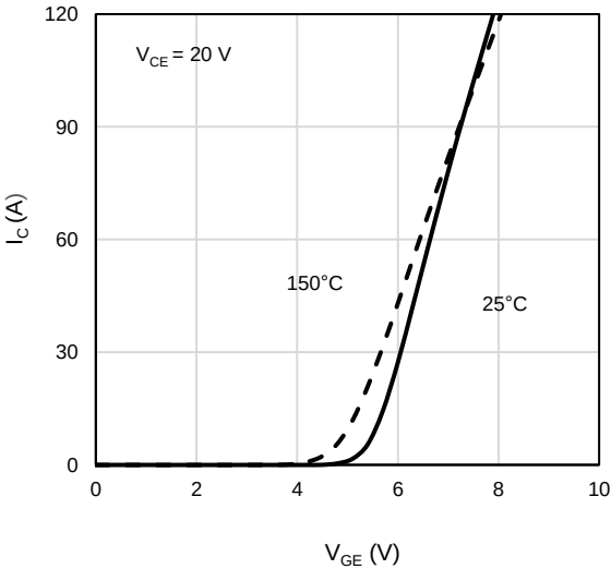
Figure 6: Transfer Characteristics
